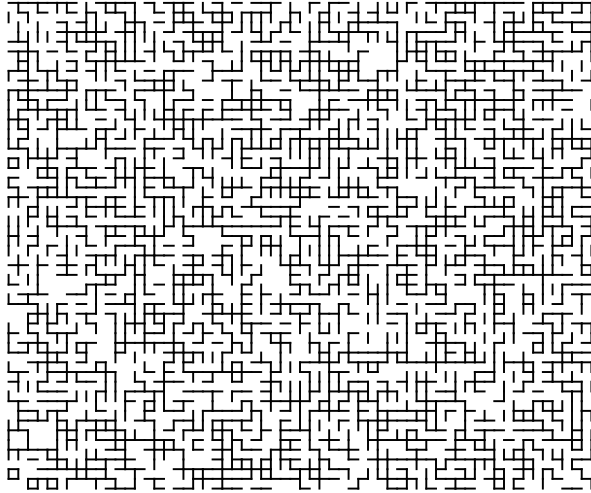
FIGURE 2. A simulation of bond percolation on \mathbb{Z}^2 in which each edge is designated ‘open’ with probability with p = 0.51 . This process is barely supercritical.
